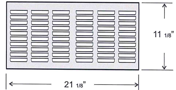
Stamped Grille
