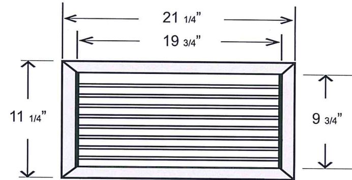
Stamped Grille
