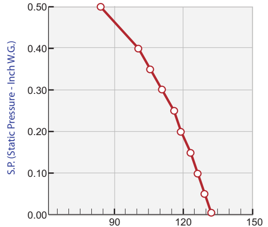
Air Flow (CFM - Cubic Feet Per Minute)
